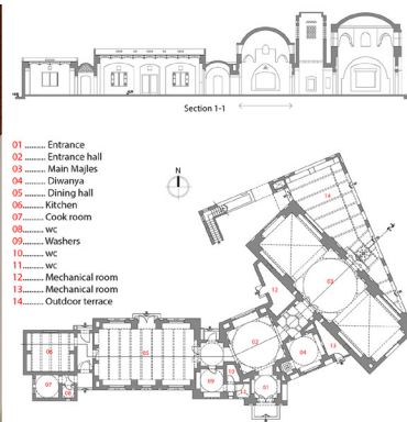
The Guest house plan & section
